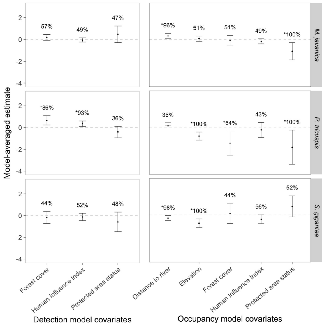
Fig. 2. Model-averaged covariate estimates for detection and occupancy, averaged across the best-supported models ( \Delta AIC_c \leq 6 ). Error bars represent 95% confidence intervals. Values above error bars indicate the percentage of candidate models in which each covariate was present. Significant covariates are denoted by an asterisk.
